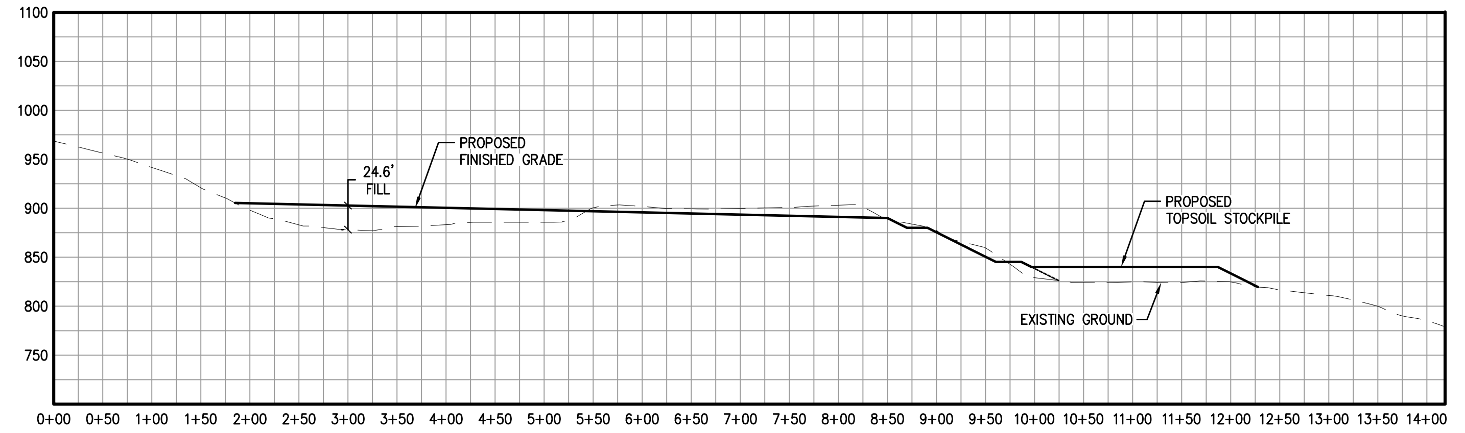
SECTION B-B SCALE: HORIZ. 1"=100' VERT. 1"=100'
