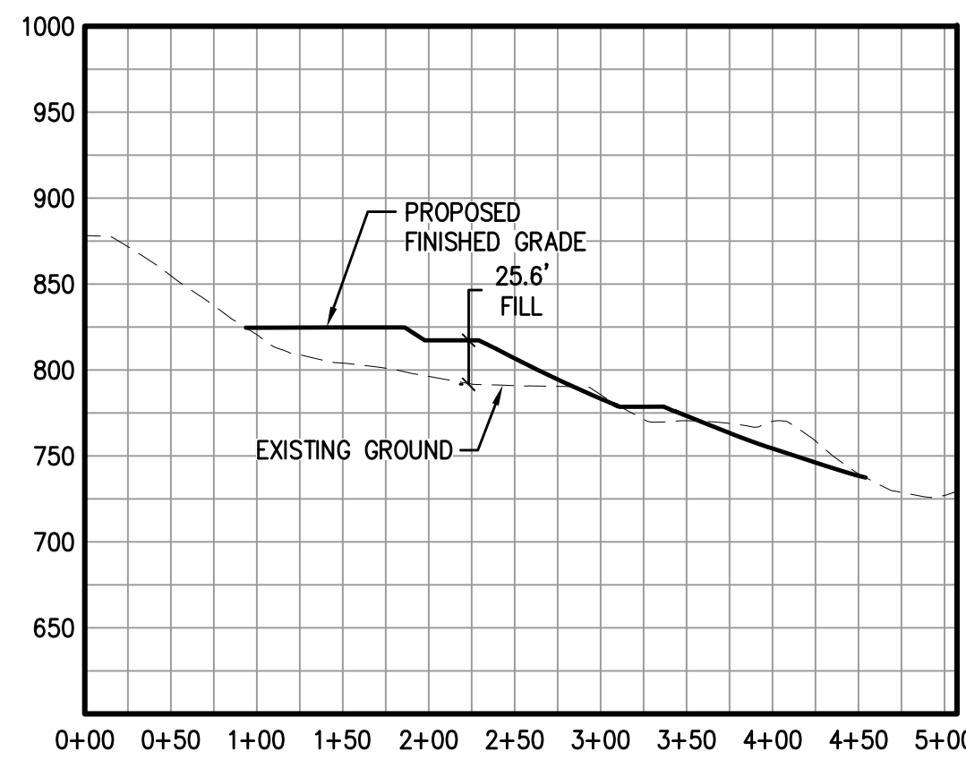
SECTION C-C SCALE: HORIZ. 1"=100' VERT. 1"=100'
