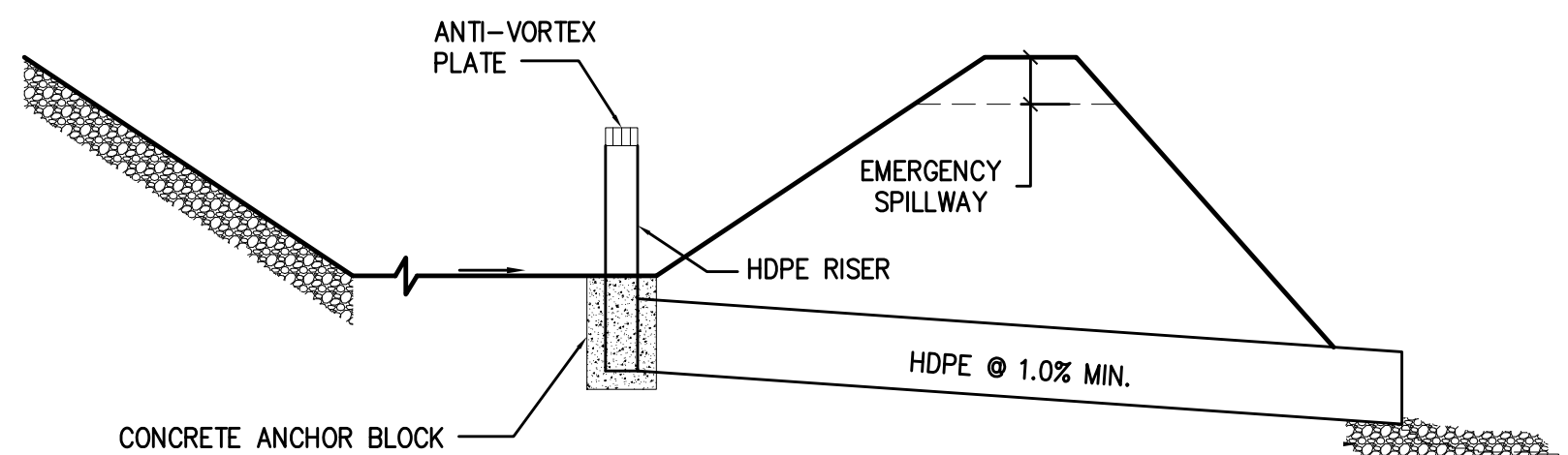
DETAIL: TYPICAL DESILTATION BASIN NOT TO SCALE
