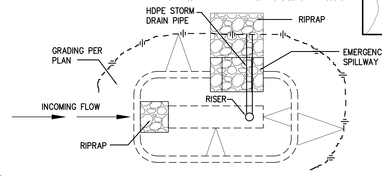
DETAIL: TYPICAL DESILTATION BASIN PLAN VIEW NOT TO SCALE
