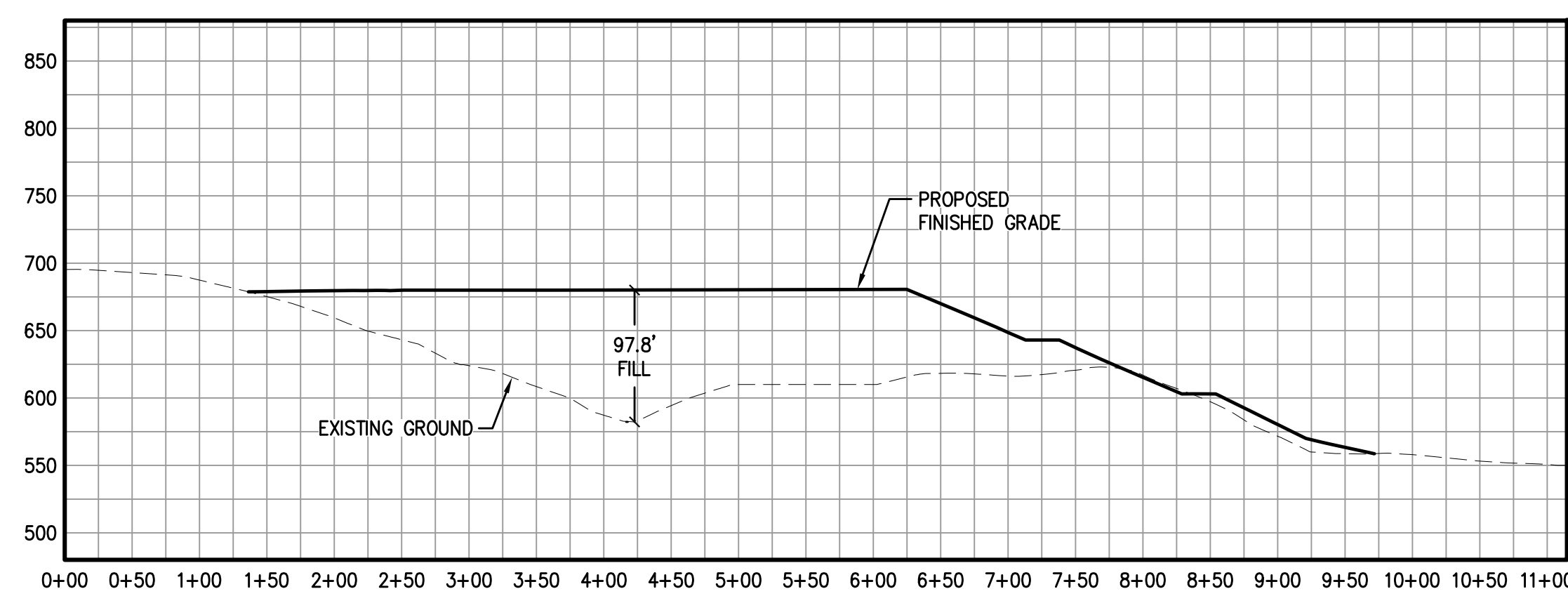
SECTION E-E SCALE: HORIZ. 1"=100' VERT. 1"=100'
