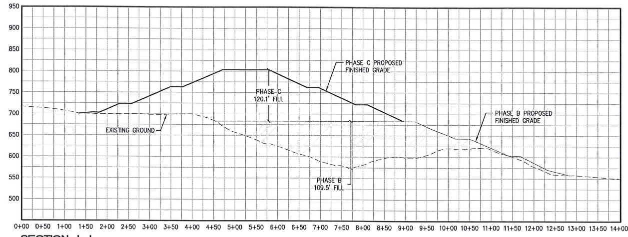
SECTION J-J SCALE: HORIZ. 1"=100' VERT. 1"=100'
