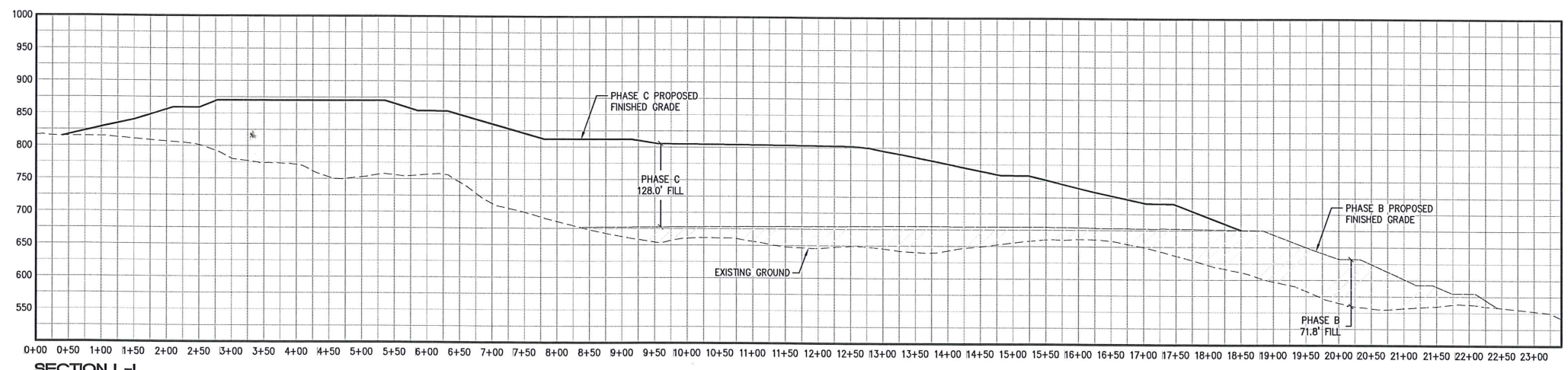
SECTION L-L SCALE: HORIZ. 1"=100' VERT. 1"=100'
