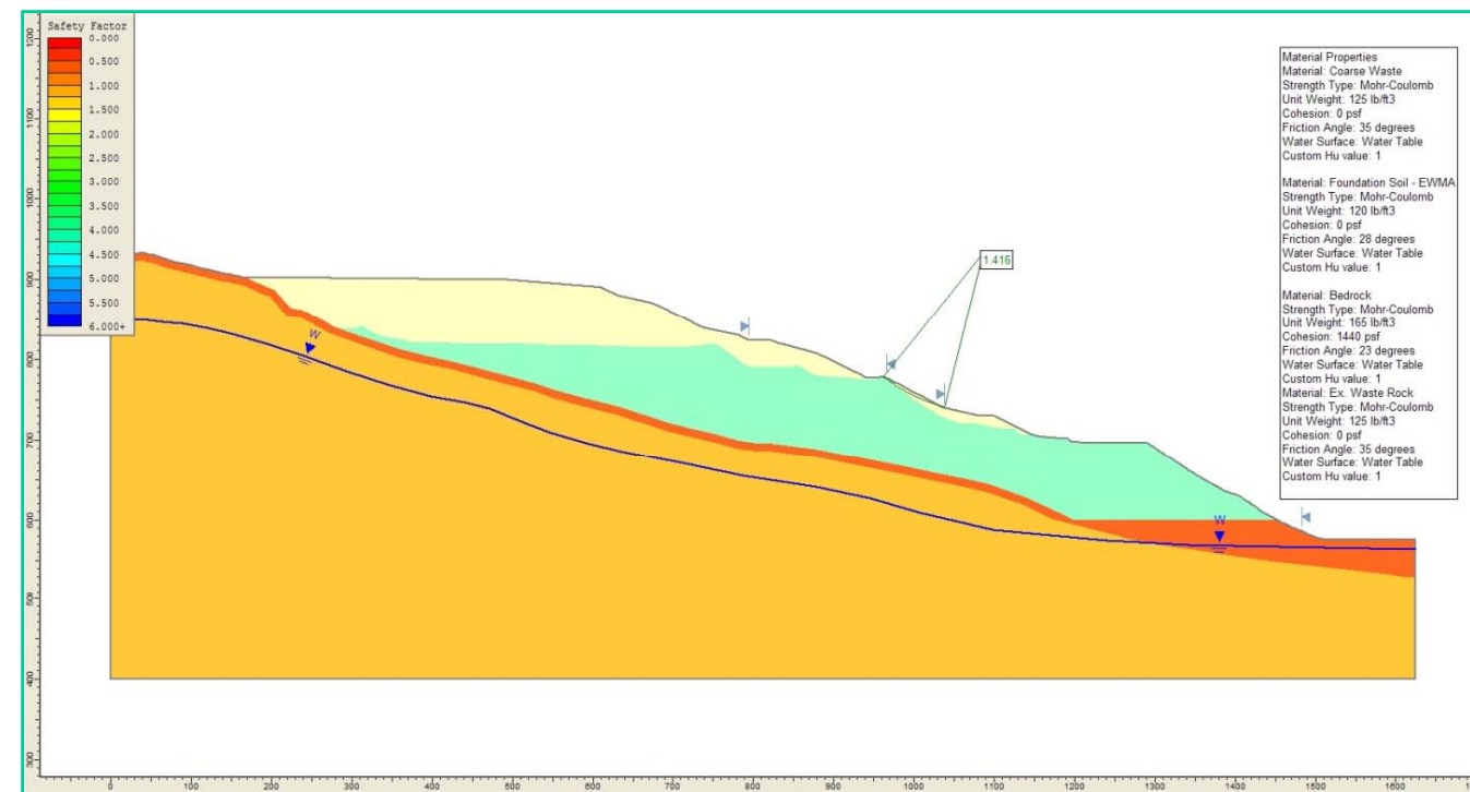
SECTION E3 –STATIC SINGLE-LIFT FAILURE (FOS = 1.42)
