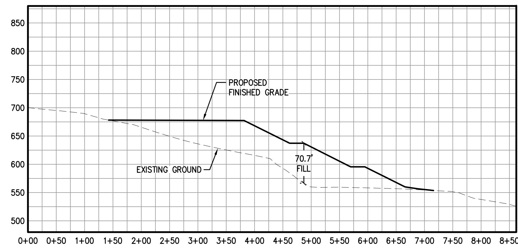
SECTION F-F SCALE: HORIZ. 1"=100' VERT. 1"=100'
