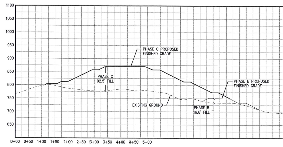
SECTION H-H SCALE: HORIZ. 1"=100' VERT. 1"=100'
