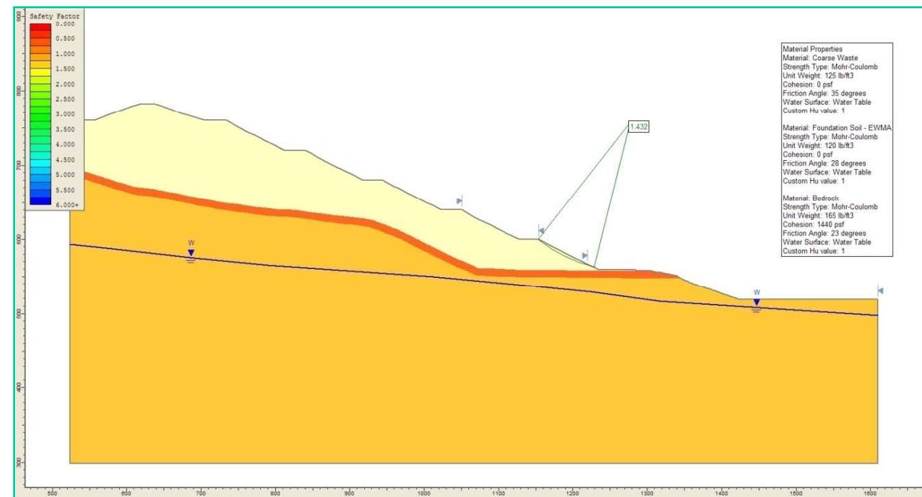
SECTION E1 – STATIC SINGLE-LIFT FAILURE (FOS = 1.43)
