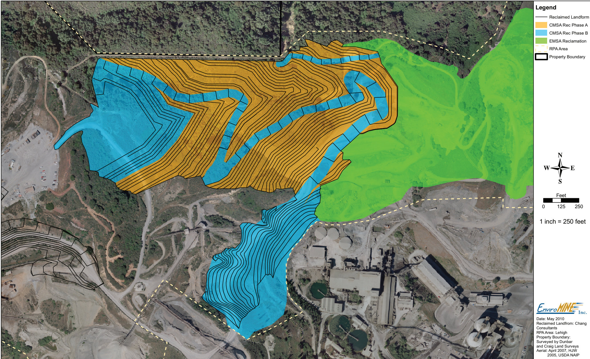
Figure 3.17-3 CMSA Reclamation Phases
