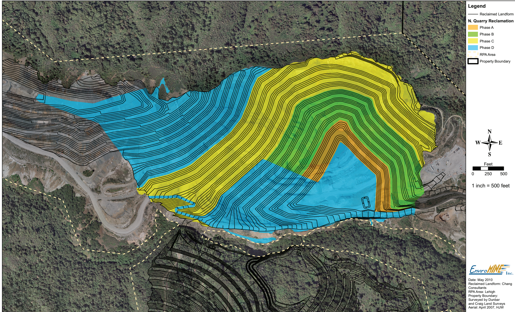
Figure 3.17-5 North Quarry Reclamation Phases
