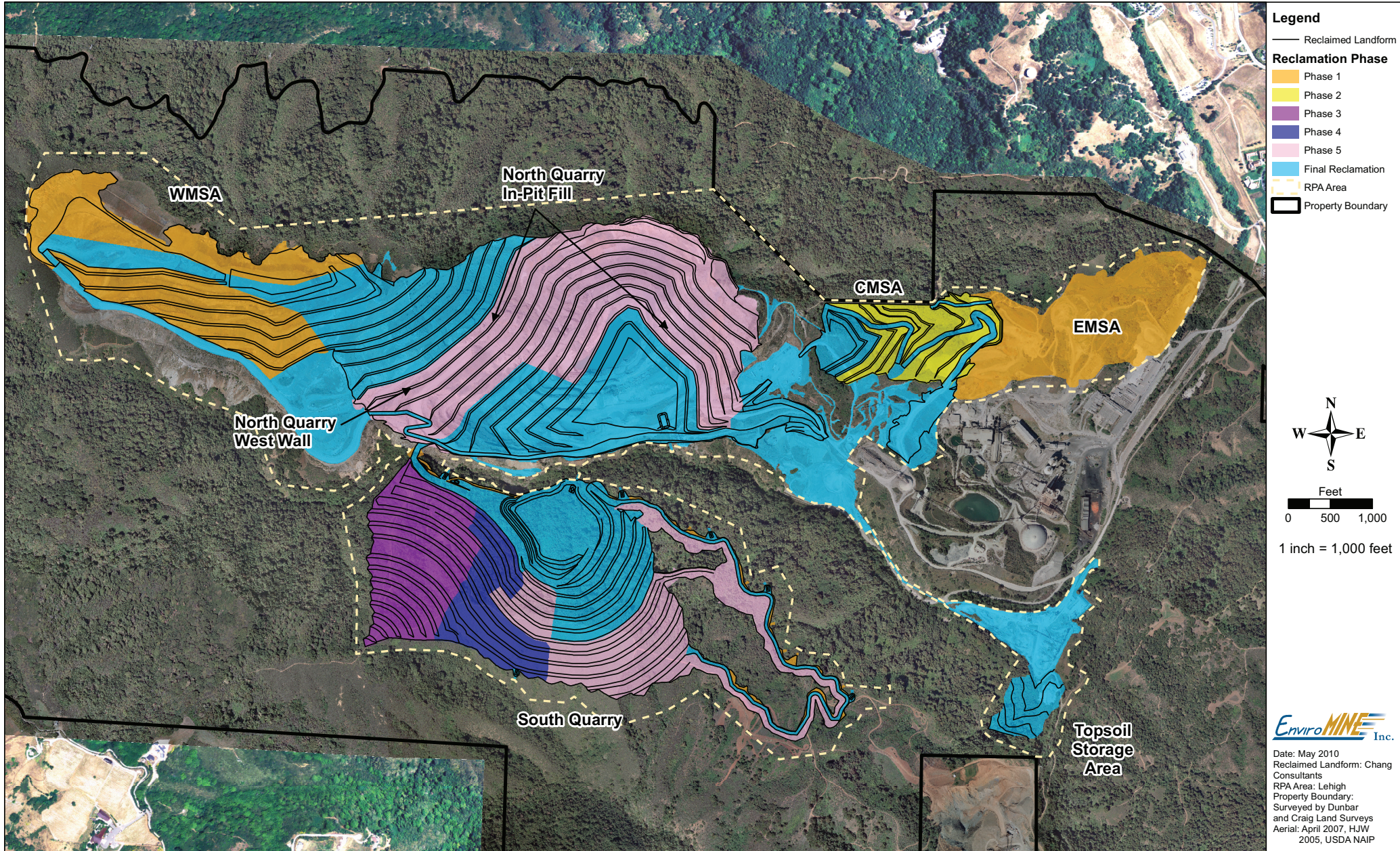
Figure 3.17-1 Reclamation Phasing Overview
