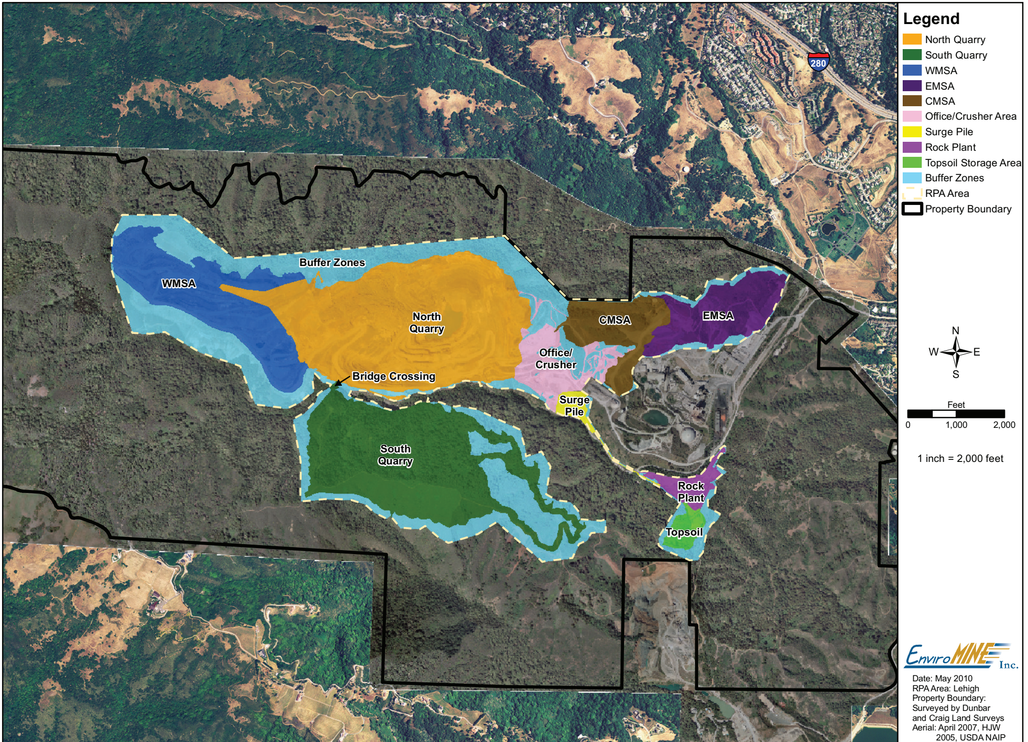
Figure 3.3-1 Quarry Components
