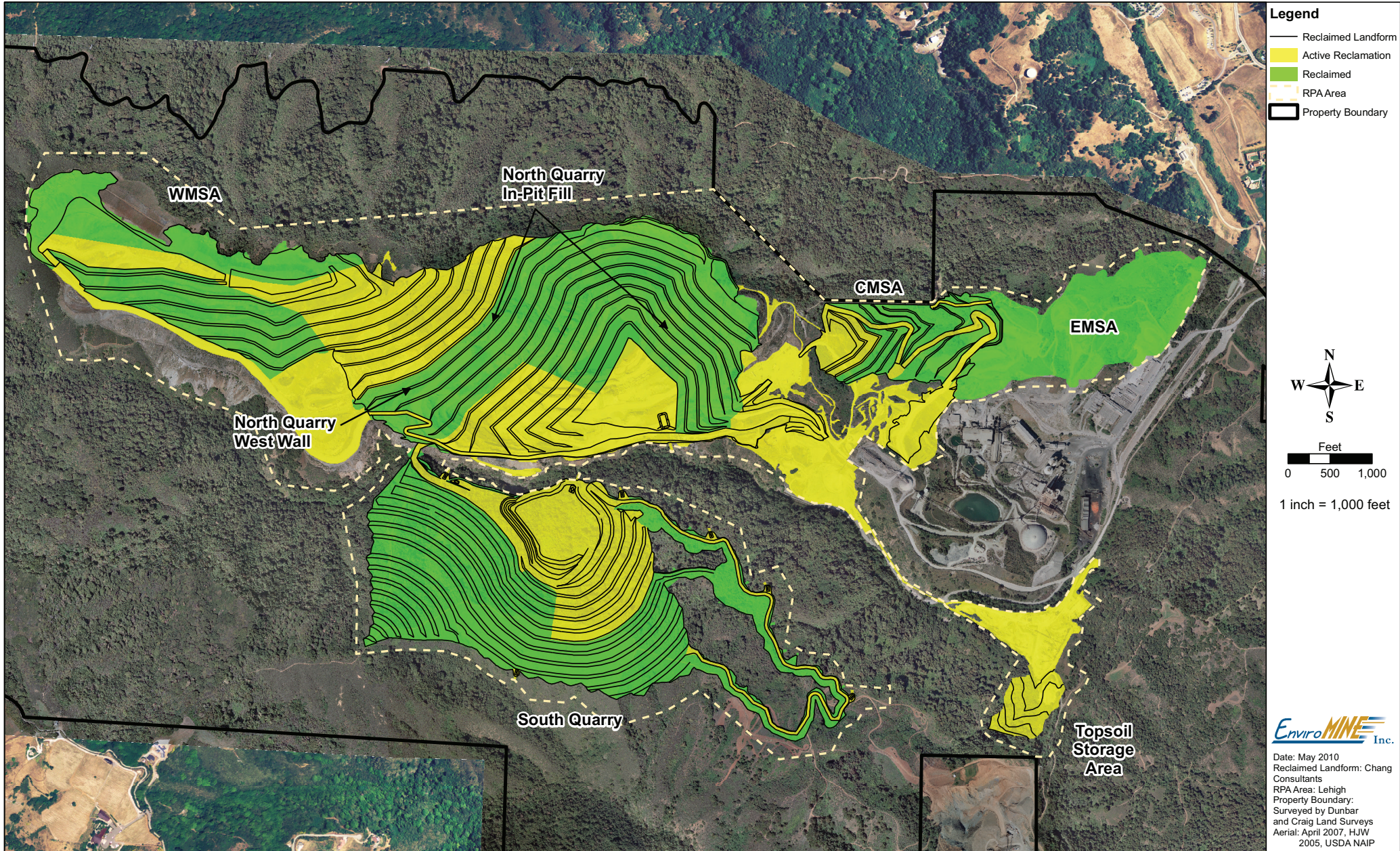
Figure 3.4-7 Final Reclamation
