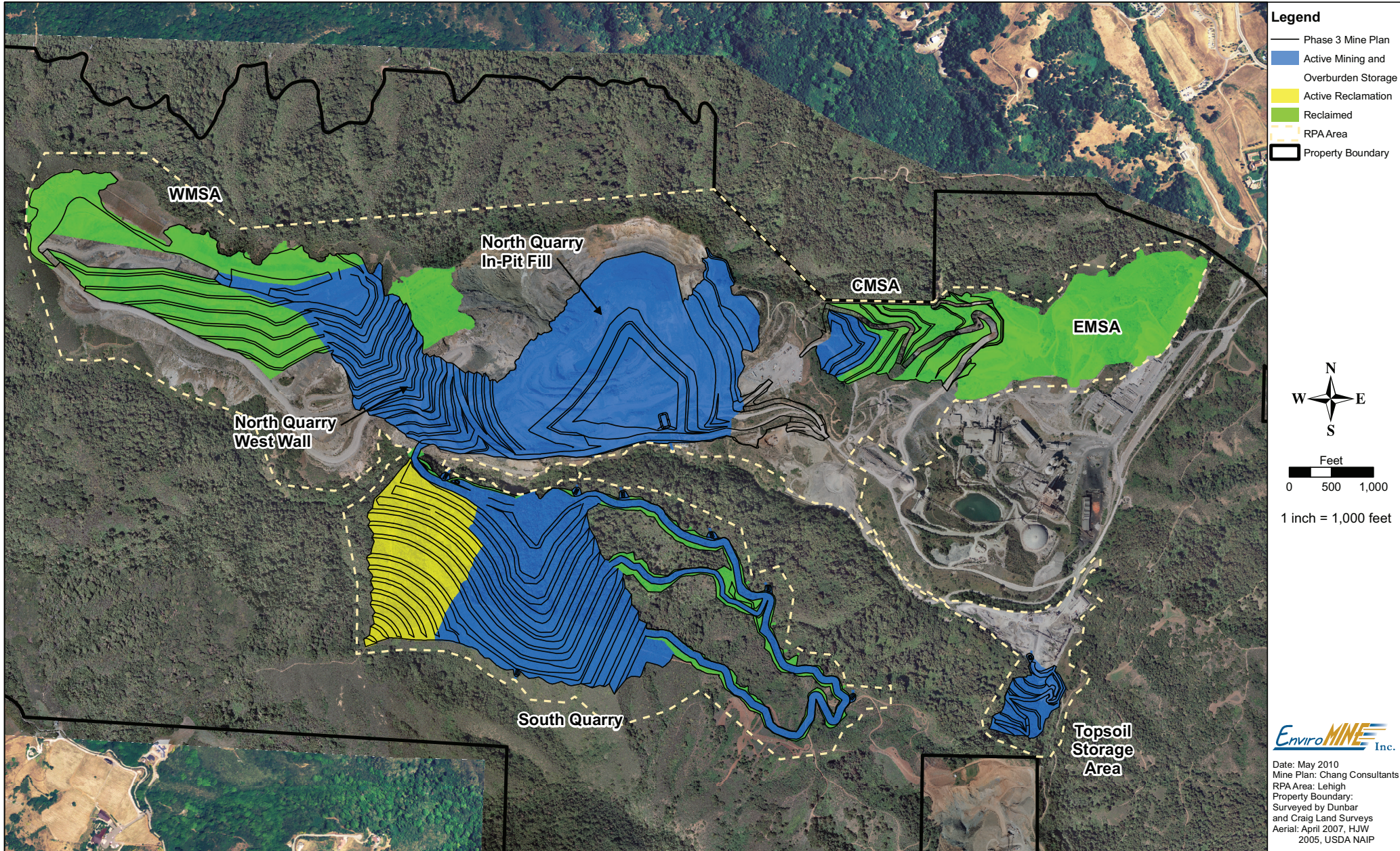
Figure 3.4-4 Mining and Reclamation Phase 3
