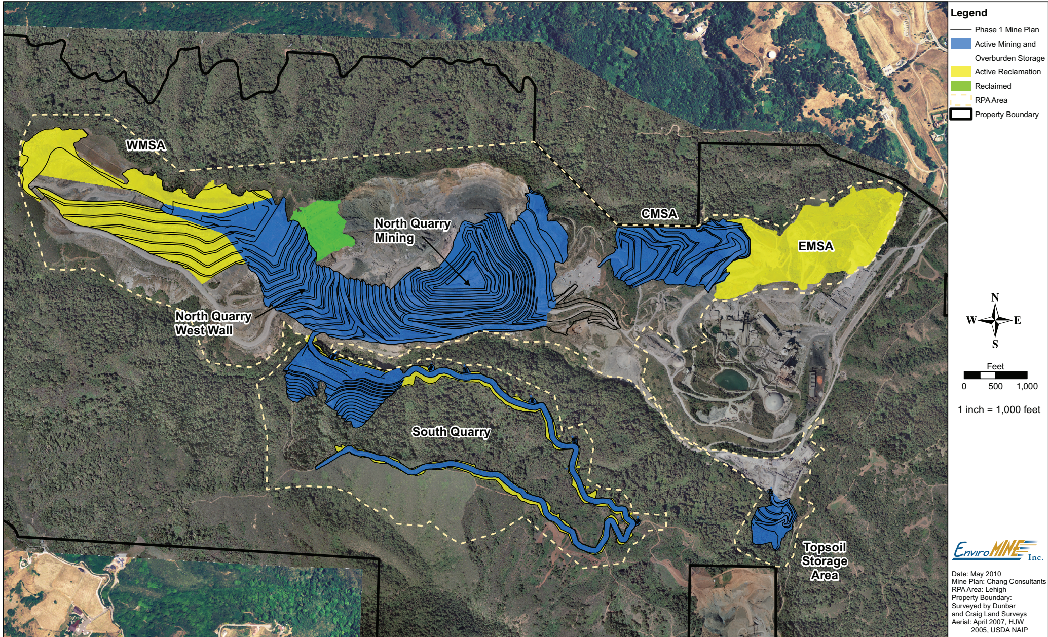
Figure 3.4-2 Mining and Reclamation Phase 1
