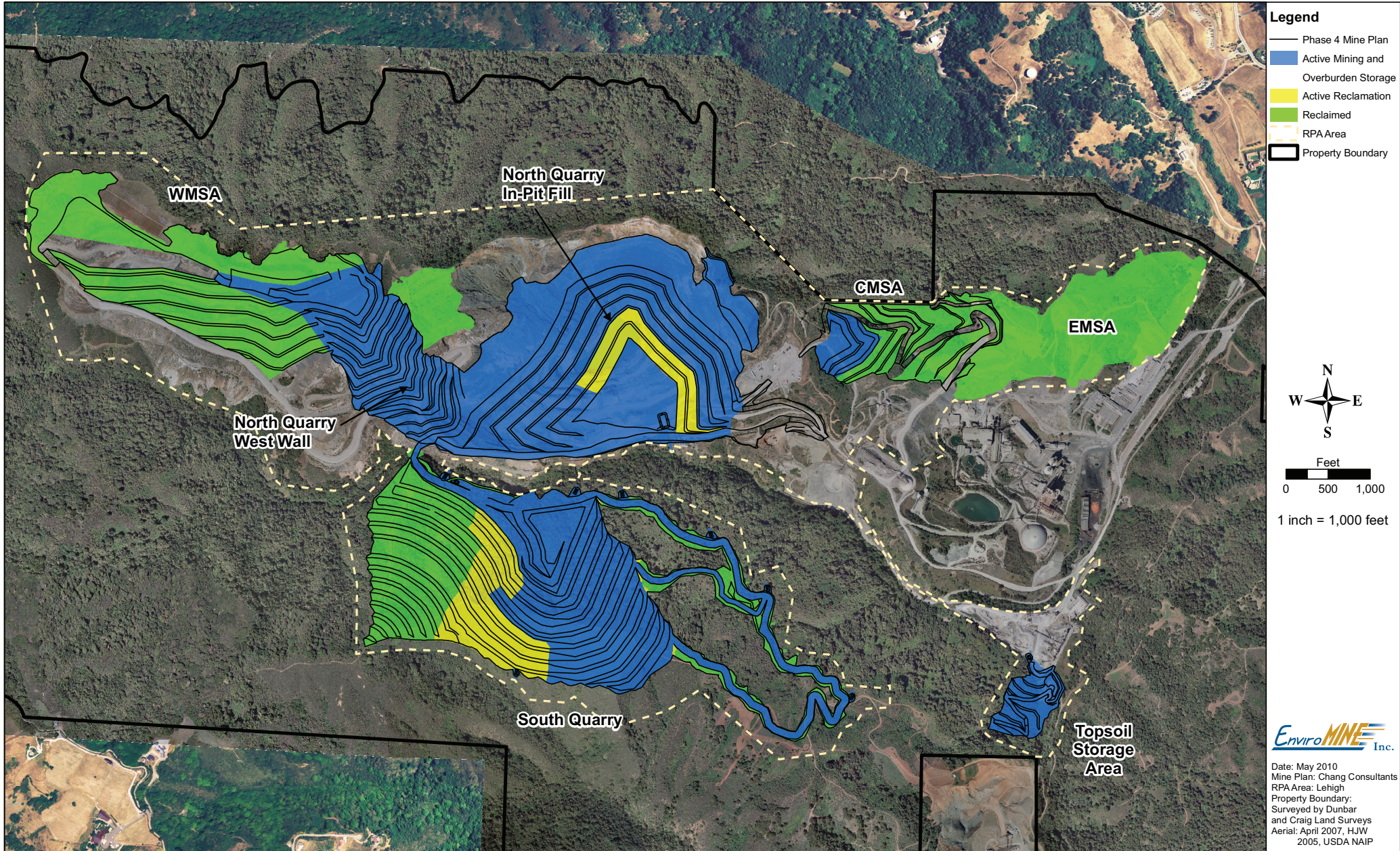
Figure 3.4-5 Mining and Reclamation Phase 4
