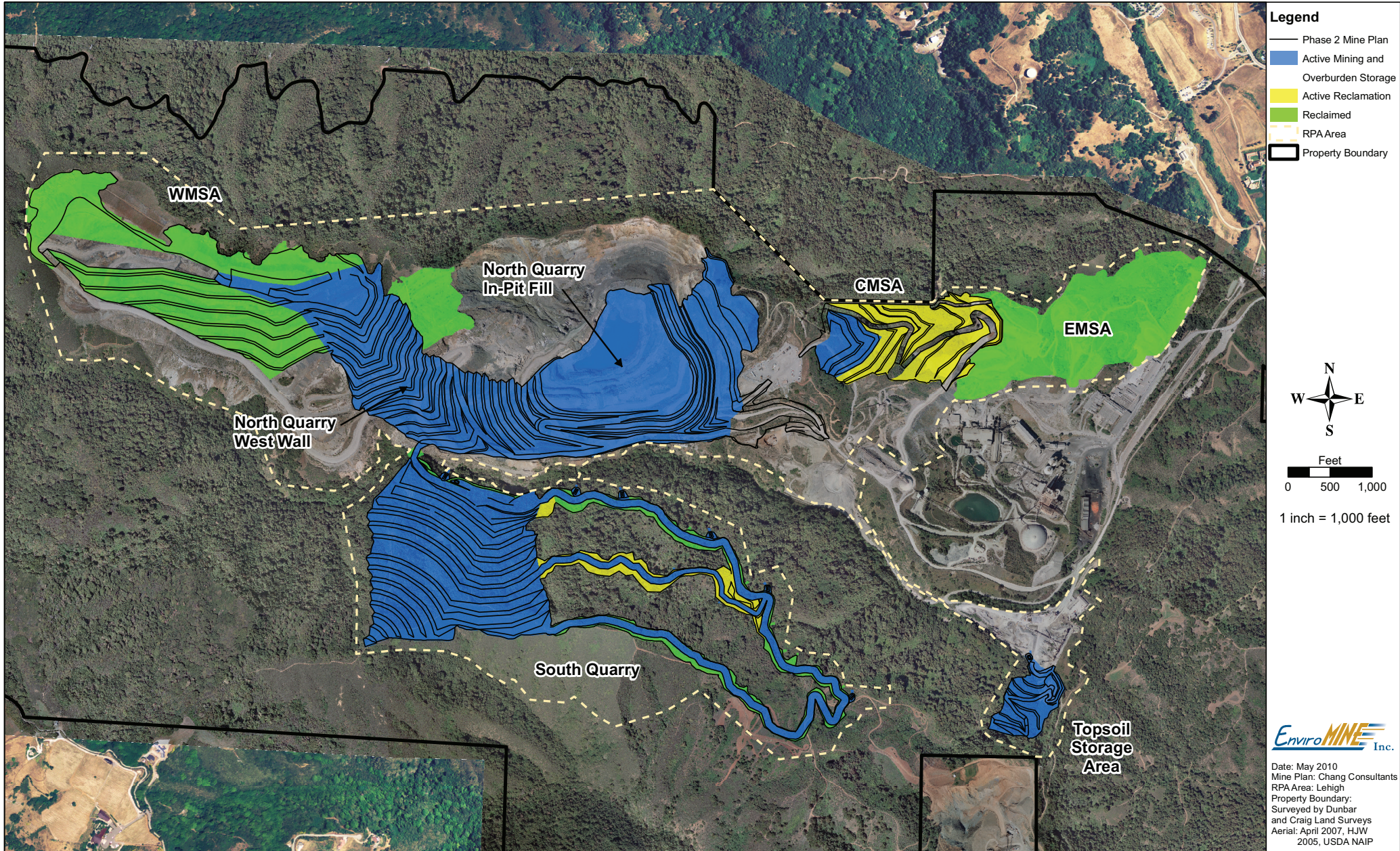
Figure 3.4-3 Mining and Reclamation Phase 2
