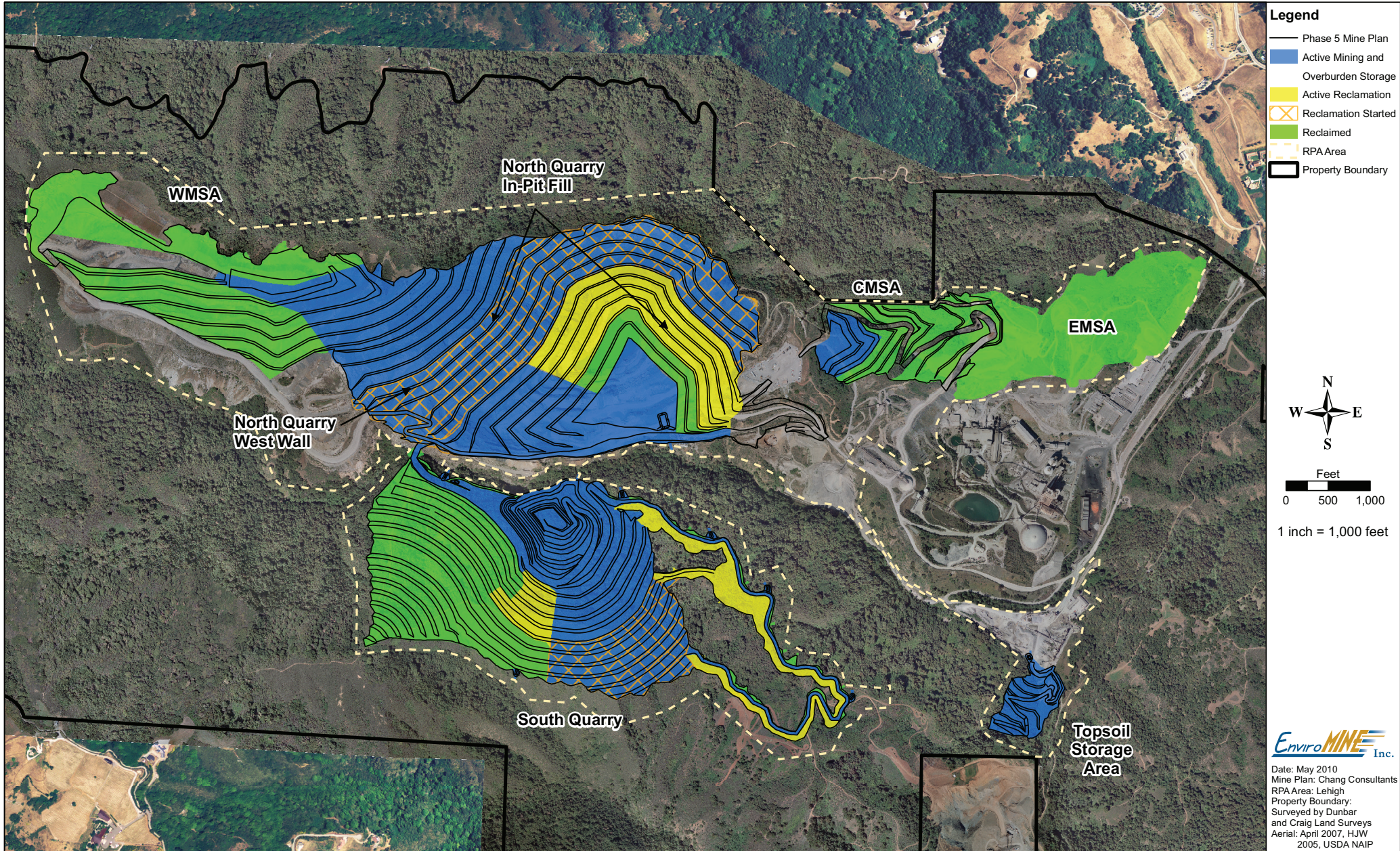
Figure 3.4-6 Mining and Reclamation Phase 5
