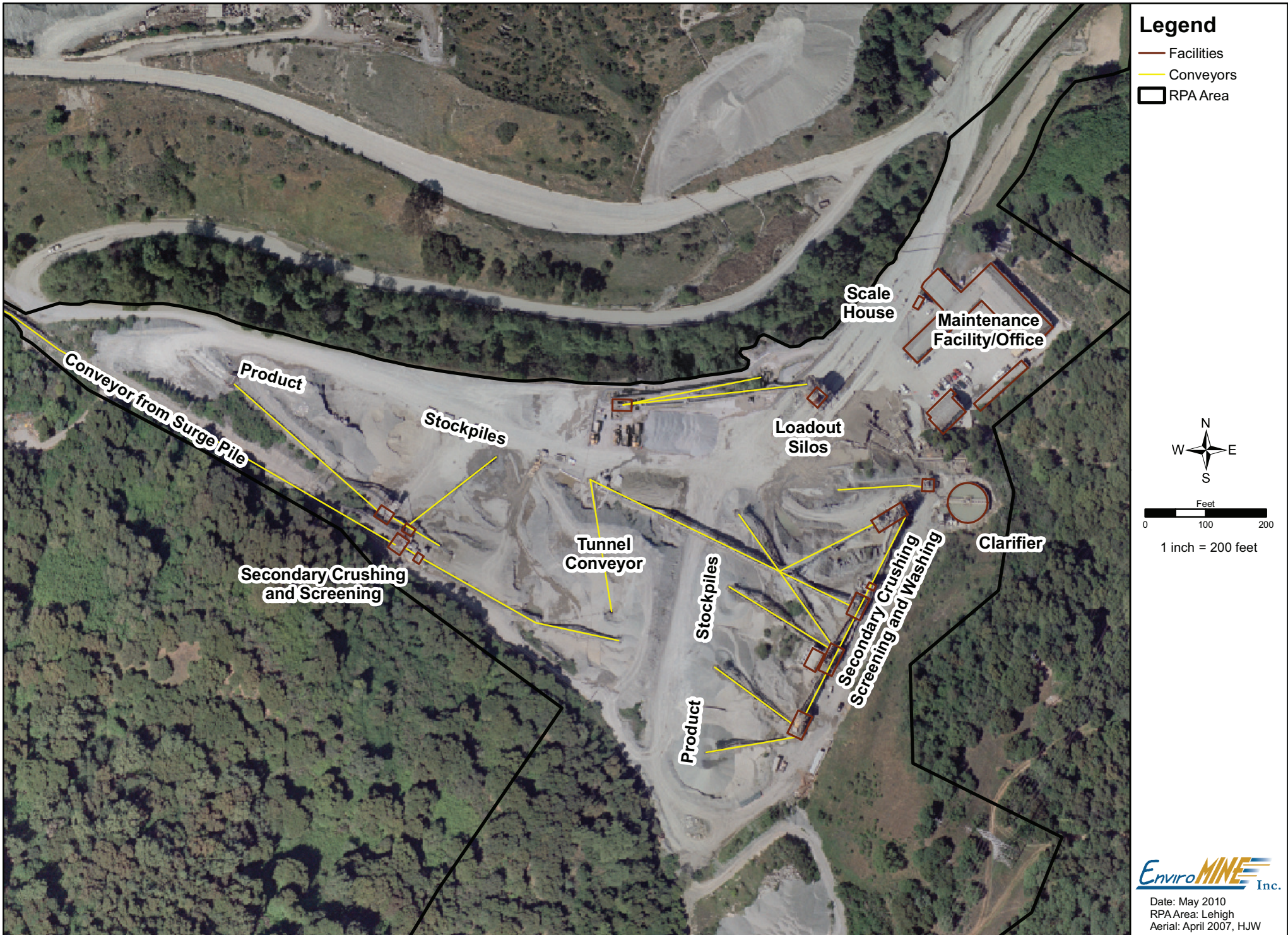
Figure 3.8-1 Rock Plant Facilities
