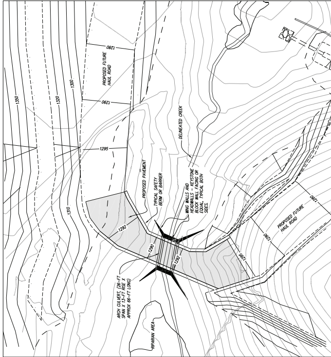
SCHMATIC LAYOUT OF PROPOSED CROSSING
