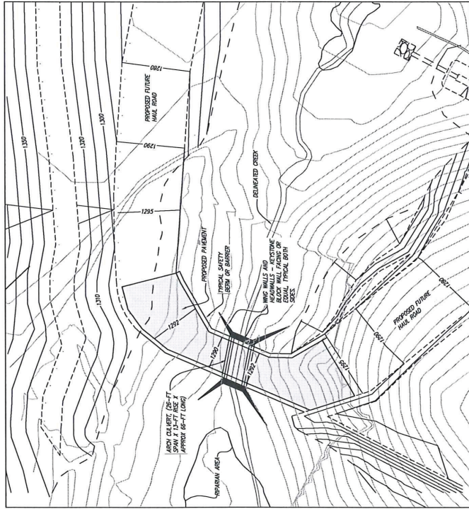
SCHEMATIC LAYOUT OF PROPOSED CROSSING
